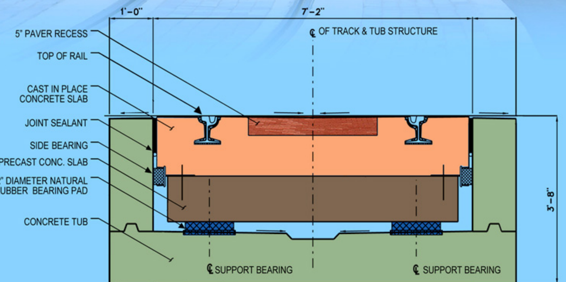
Cross Section of Floating Track Slab
